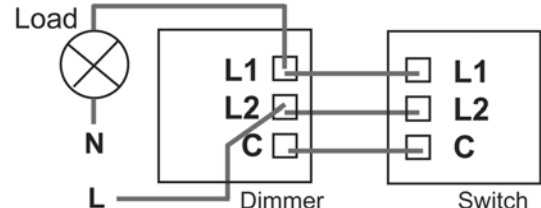
Figure 3. Using a 2-way Dimmerswitch.
