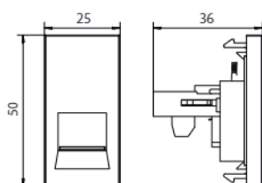
EMRJ11x
