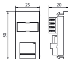
EMRJ45C5Ex
