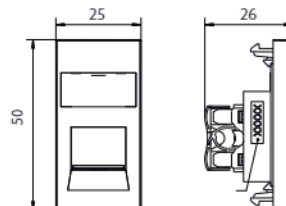
EMRJ45C6x
